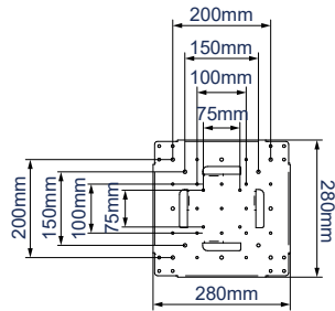
VESA INTERFACE PLATE
