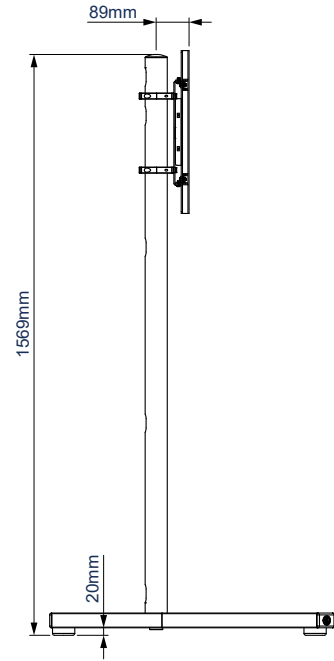
SIDE VIEW WITH LEVELLING FEET
