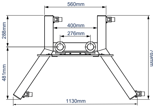
TROLLEY BASE
