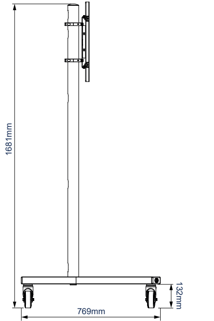
SIDE VIEW WITH CASTORS
