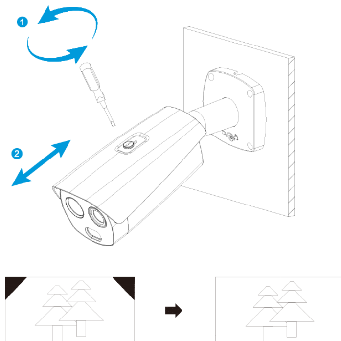
Figure 4-4 Adjusting sun shield cover
