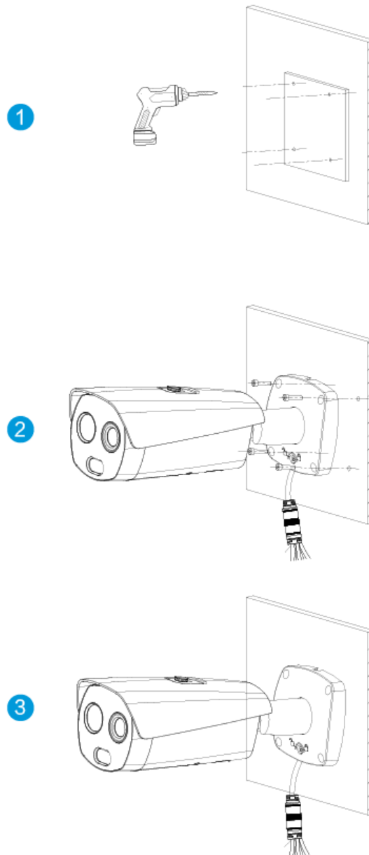
Figure 4-2 Fixing camera
