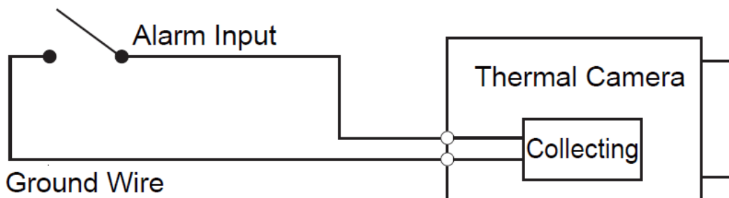
Figure 5-2 Alarm input
