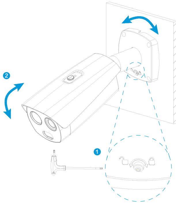
Figure 4-5 Adjusting camera
