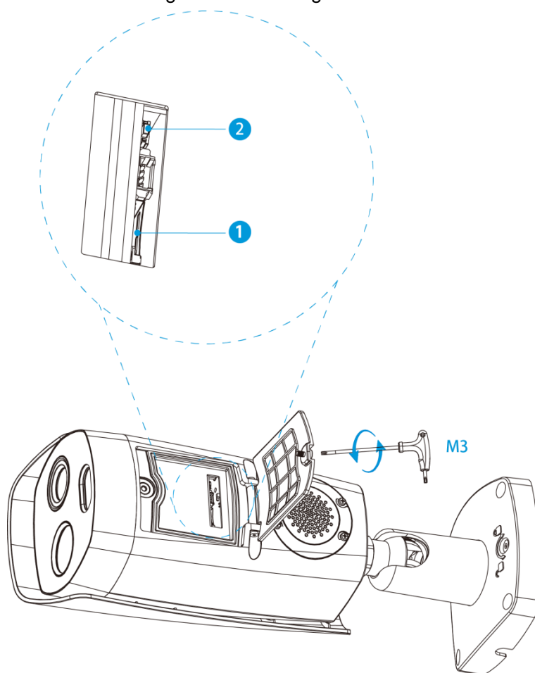
Figure 4-1 Installing SD card
