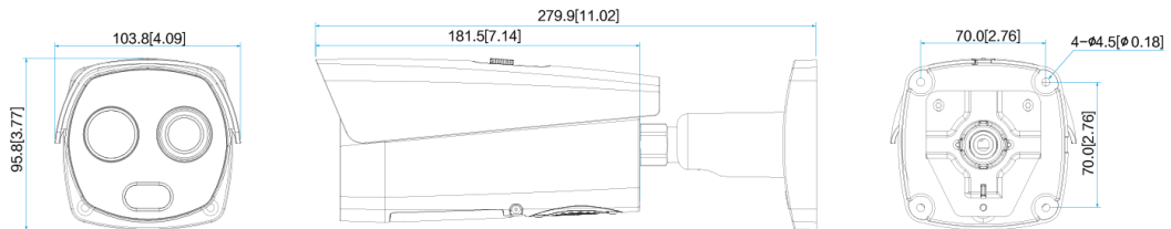
Figure 2-1 Dimensions (mm [inch])
