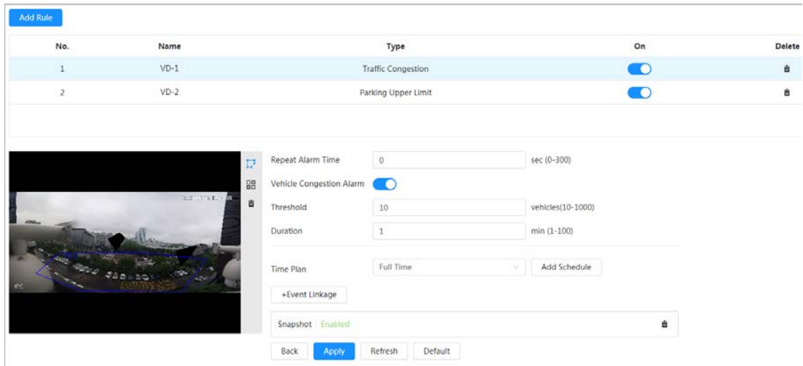
Figure 8-25 Vehicle density (traffic congestion)
