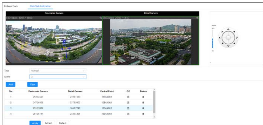
Figure 8-65 Manual calibration
