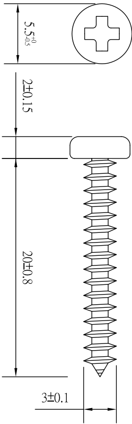
M3 x 20 Hardware Installation
